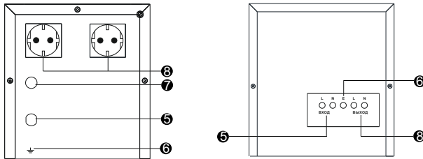
Rear panel
